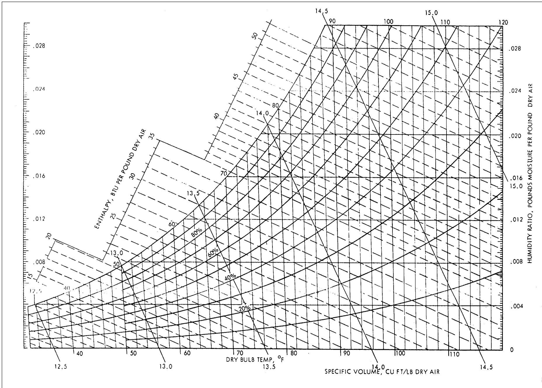
Figure 2. A psychrometric chart.
