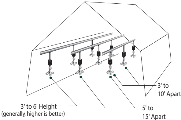
Typical Installation for Humidification or Cooling
